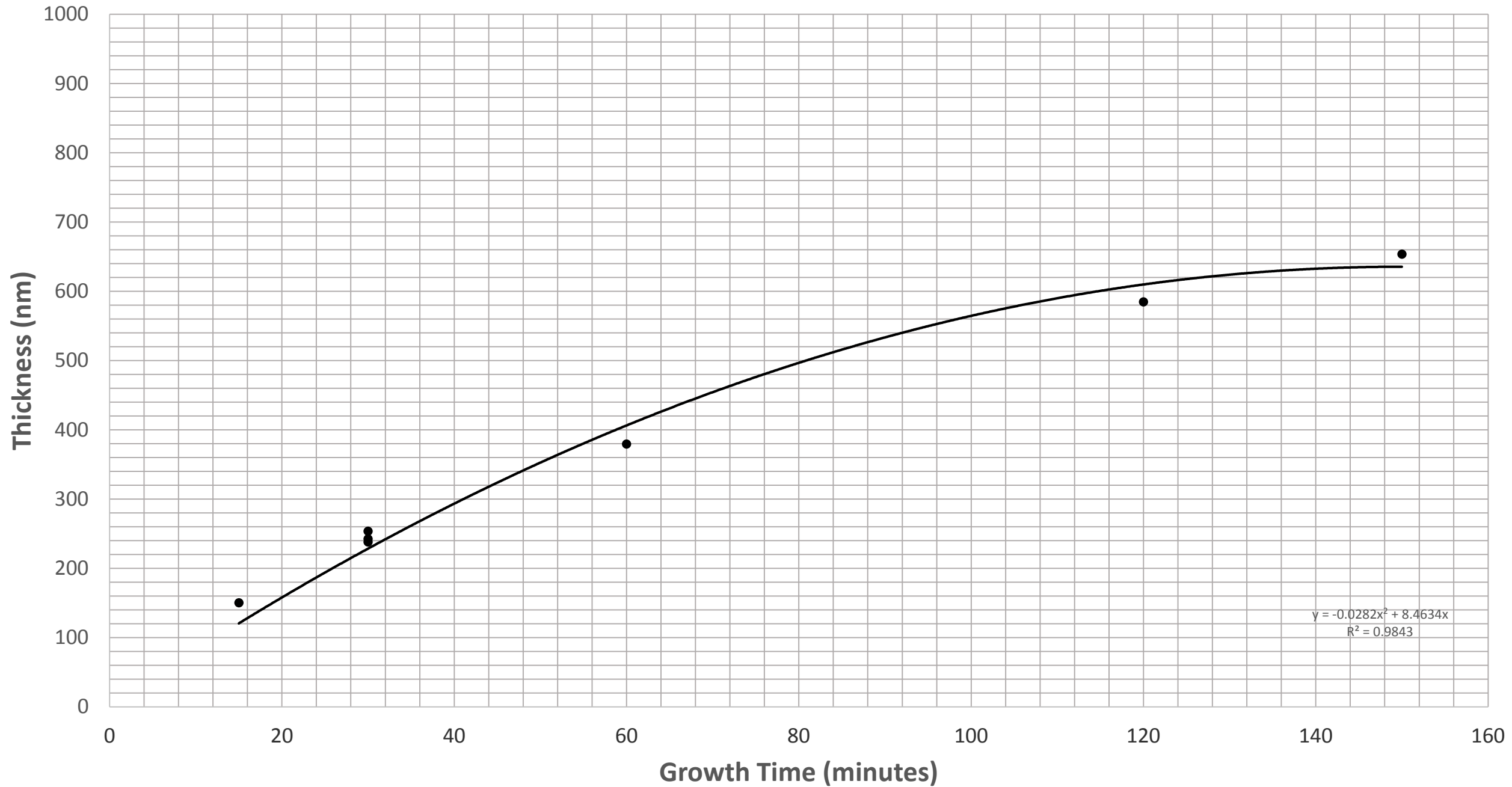
CVD 1034 Wet Oxidation Growth Thickness at 1050 °C, n-type, (100) Si
